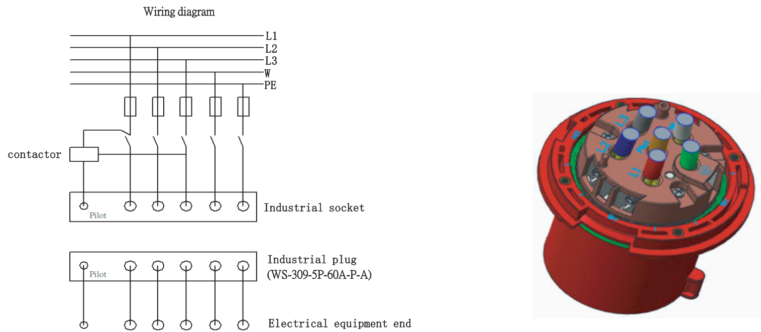
Fig.4 Wiring diagram
