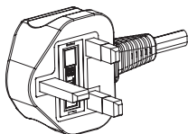
WS-012A-A (small body) (Flat SR) With fuse
