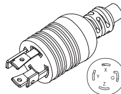
WS-131 NEMA L15-30P
