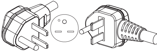
WS-001Q NEMA 6-30P
