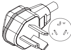
WS-001J NEMA 10-30P
