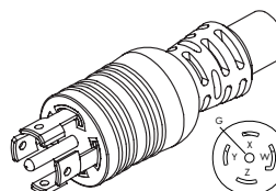
WS-224 NEMA L22-30P
