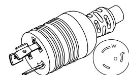
WS-330 NEMA L7-20P
