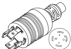
WS-122 NEMA L14-30P
