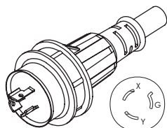
WS-123-2 NEMA L6-15P
