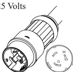
WS-266-3 NEMA SS1-50P
