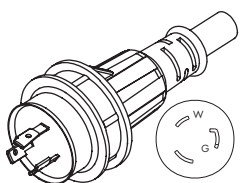
WS-117-2 NEMA L5-20P
