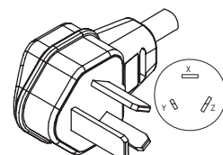
WS-001U NEMA 11-50P
