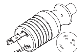
WS-121-5 NEMA L5-30P
