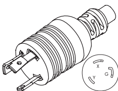
WS-120 NEMA L6-30P
