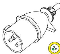
WS-197-P2 2P3W-16A-4H 100-130V~
