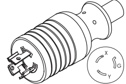
WS-123-5 NEMA L6-15P
