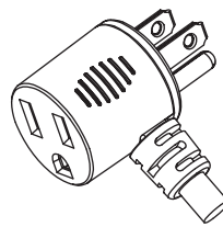
*WS-022D Ultrasonic welding, Without Ear 8-Position angle plug
