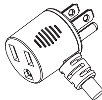
*WS-022BD Ultrasonic welding, Without Ear 8-Position angle plug
