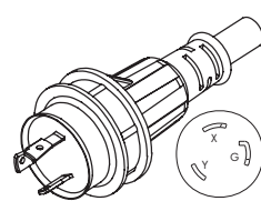
WS-120-2 NEMA L6-30P
