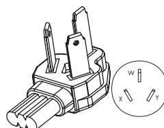
WS-001J1-2 (Small body) NEMA 10-50P
