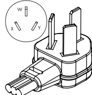
WS-001J1-1 (Economic Body) NEMA 10-50P
