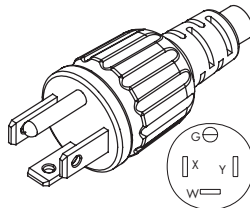
WS-001-3 NEMA 14-20P
