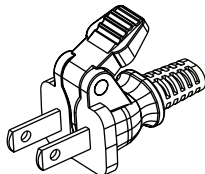
WS-004-W Easy Pull Smart Plug Ultrasonic Welding Assembly
