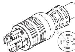
WS-225 NEMA L21-30P
