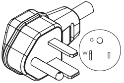
WS-001L NEMA 5-50P
