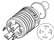
WS-122-5 NEMA L14-30P
