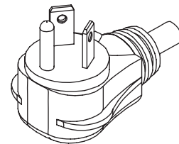
WS-001X-2 NEMA 7-20P
