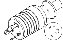
WS-117-5 NEMA L5-20P
