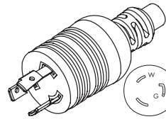
WS-117 NEMA L5-20P
