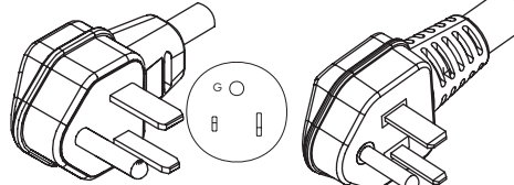
WS-001N NEMA 6-50P
