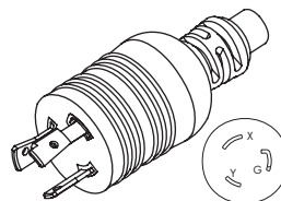
WS-119 NEMA L6-20P
