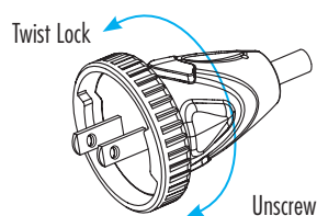
WS-004-11 Twist and Lock Secure System
