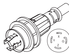
WS-131-2 NEMA L15-30P
