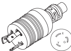
WS-119 NEMA L6-20P
