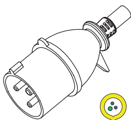
WS-196-1-P2 2P3W-32A-4H 100-130V~
