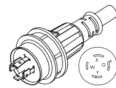
WS-129-2 NEMA L14-20P
