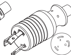
WS-120-5 NEMA L6-30P
