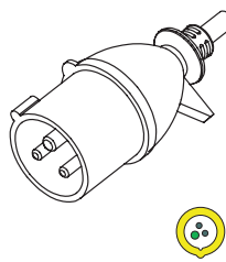
WS-197 2P3W-16A-4H 100-130V~
